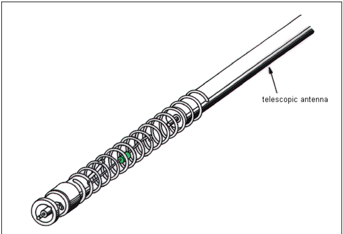
Figure 13.9 Final assembly of the antenna.
