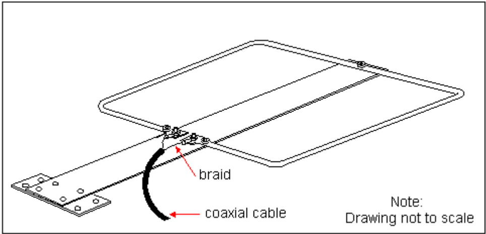
Figure 7.10 Connecting the coaxial cable to the loop element.
