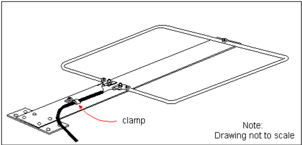
Figure 7.11 Clamping the coaxial cable to the plastic mount.
