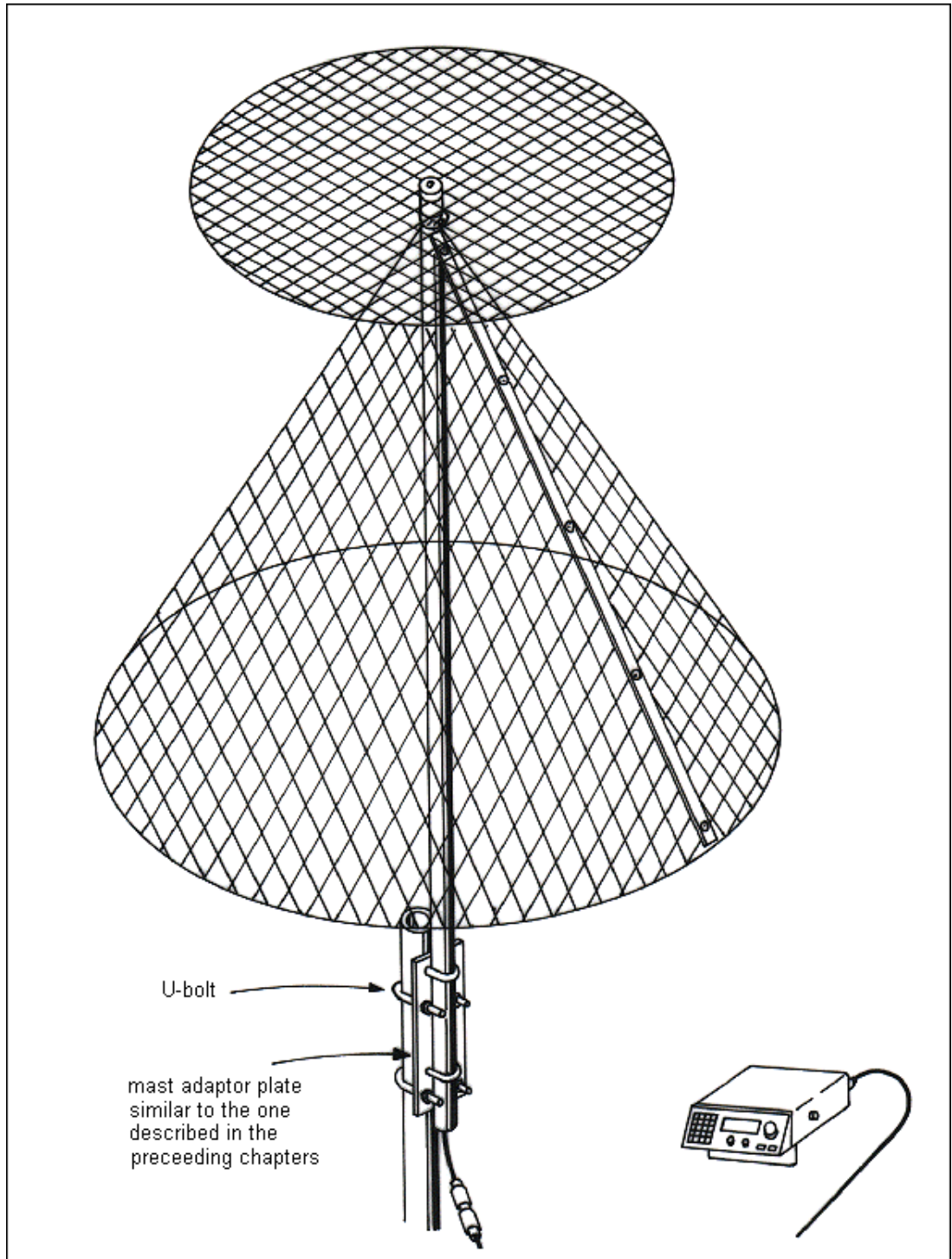
Figure 8.19 Mounting the CD-2W to the mast.
